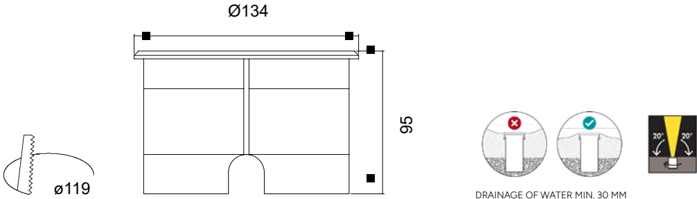
DRAINAGE OF WATER MIN. 30 MM
