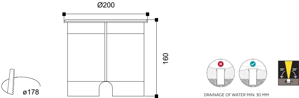
DRAINAGE OF WATER MIN. 30 MM
