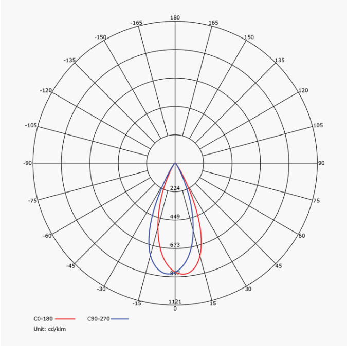
Diagrama polar 45°. Polar intensity diagram 45°
