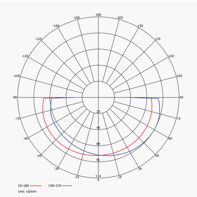
Diagrama polar 15°. Polar intensity diagram 15°
